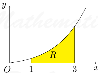
Figure 2: y = xe^x
