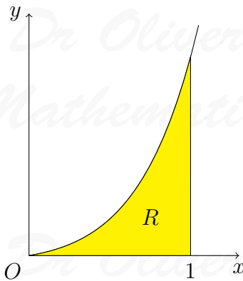
Figure 1: y = xe^{2x}
